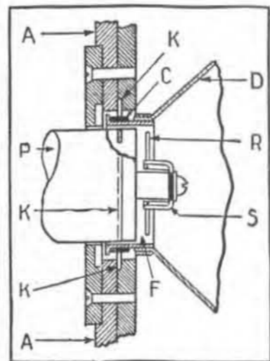
A new design of coil-driven loud speaker, which uses copper rings as a short-circuited secondary winding of the moving coil, to reduce the effective impedance at higher frequencies.
